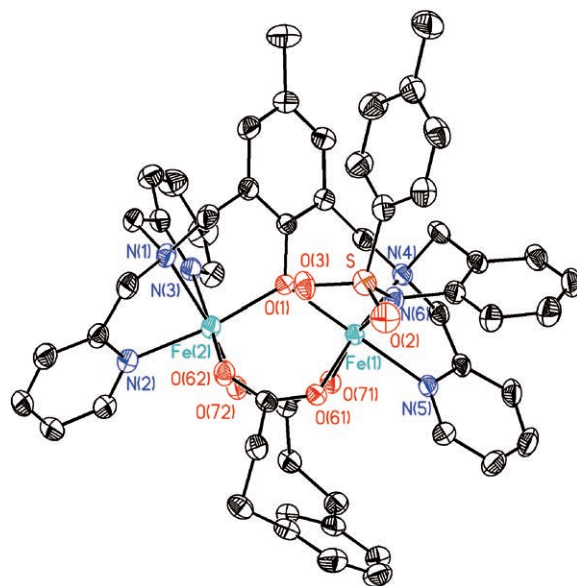
Figure 3. X-ray crystal structure of the dication 3a [\text{Fe}_2(\text{L-H+NHTs})(\text{mpdp})]^{2+} (ellipsoids are set at 30% probability, and hydrogen atoms are omitted for clarity). Fe–ligand bond lengths [Å]: Fe(1)–O(61) 1.9639(17), Fe(1)–O(1) 2.0161(16), Fe(1)–N(6) 2.016(2), Fe(1)–O(71) 2.1230(18), Fe(1)–N(5) 2.130(2), Fe(1)–N(4) 2.182(2), Fe(2)–O(72) 1.9370(17), Fe(2)–O(62) 1.9909(19), Fe(2)–O(1) 2.0161(16), Fe(2)–N(3) 2.127(2), Fe(2)–N(2) 2.129(2), Fe(2)–N(1) 2.178(2), Fe(1)–Fe(2) 3.462.
