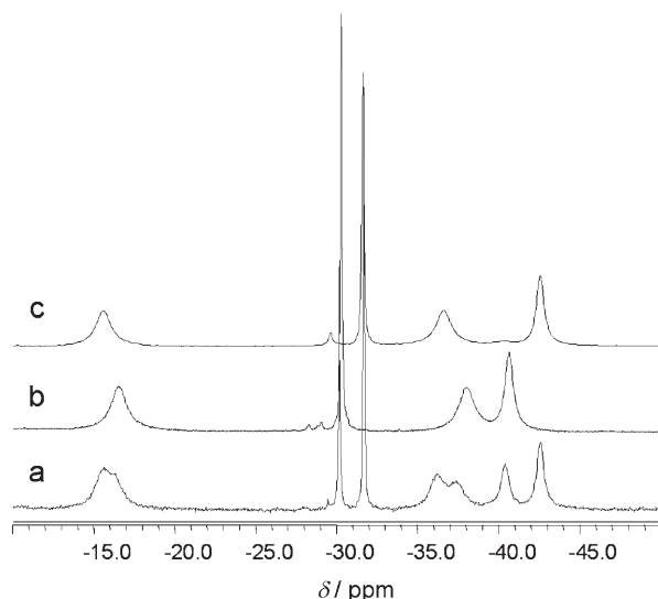
Figure 2. ^1\text{H} NMR spectra of the iodide-reduced reaction mixture (a) and complexes 3a (b) and 3b (c) in \text{CD}_3\text{CN} over the -10 to -50 ppm range.
